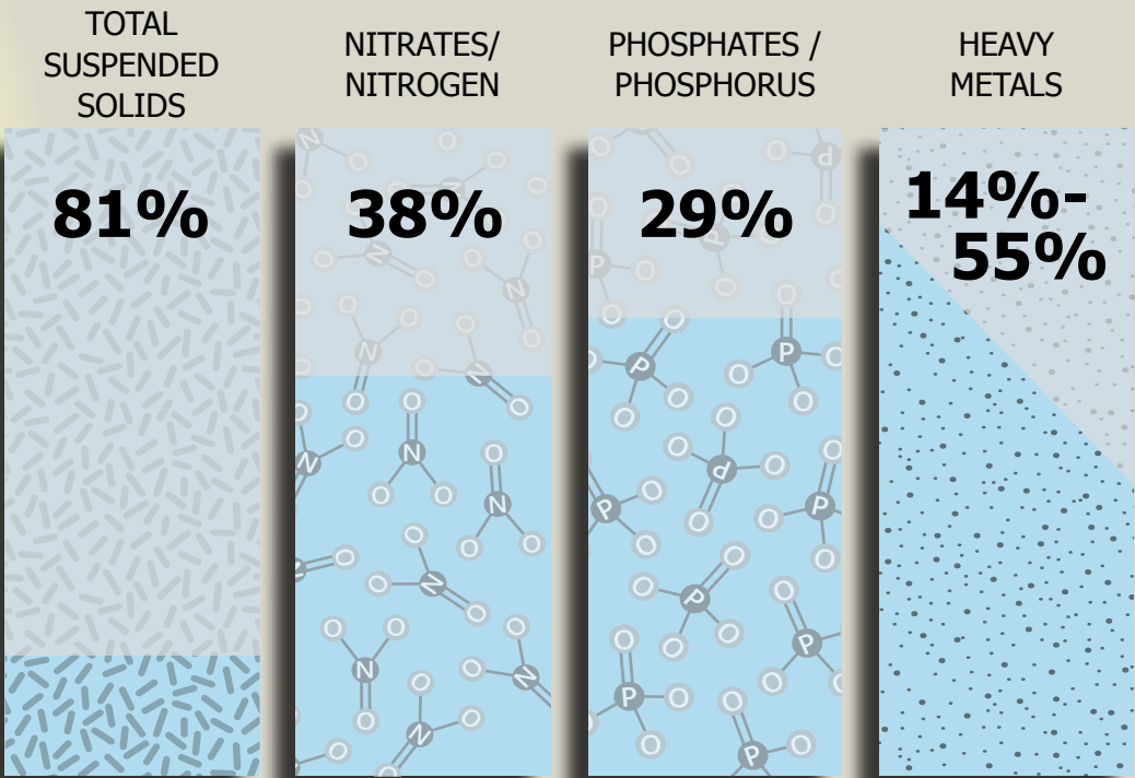
Source: EPA NPDES Menu of BMPs - Grassed Swales, 1997
