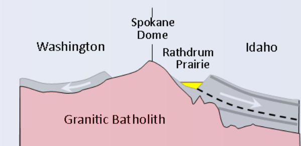
Batholith emplacement displaces Belt Supergroup rocks to east and west
