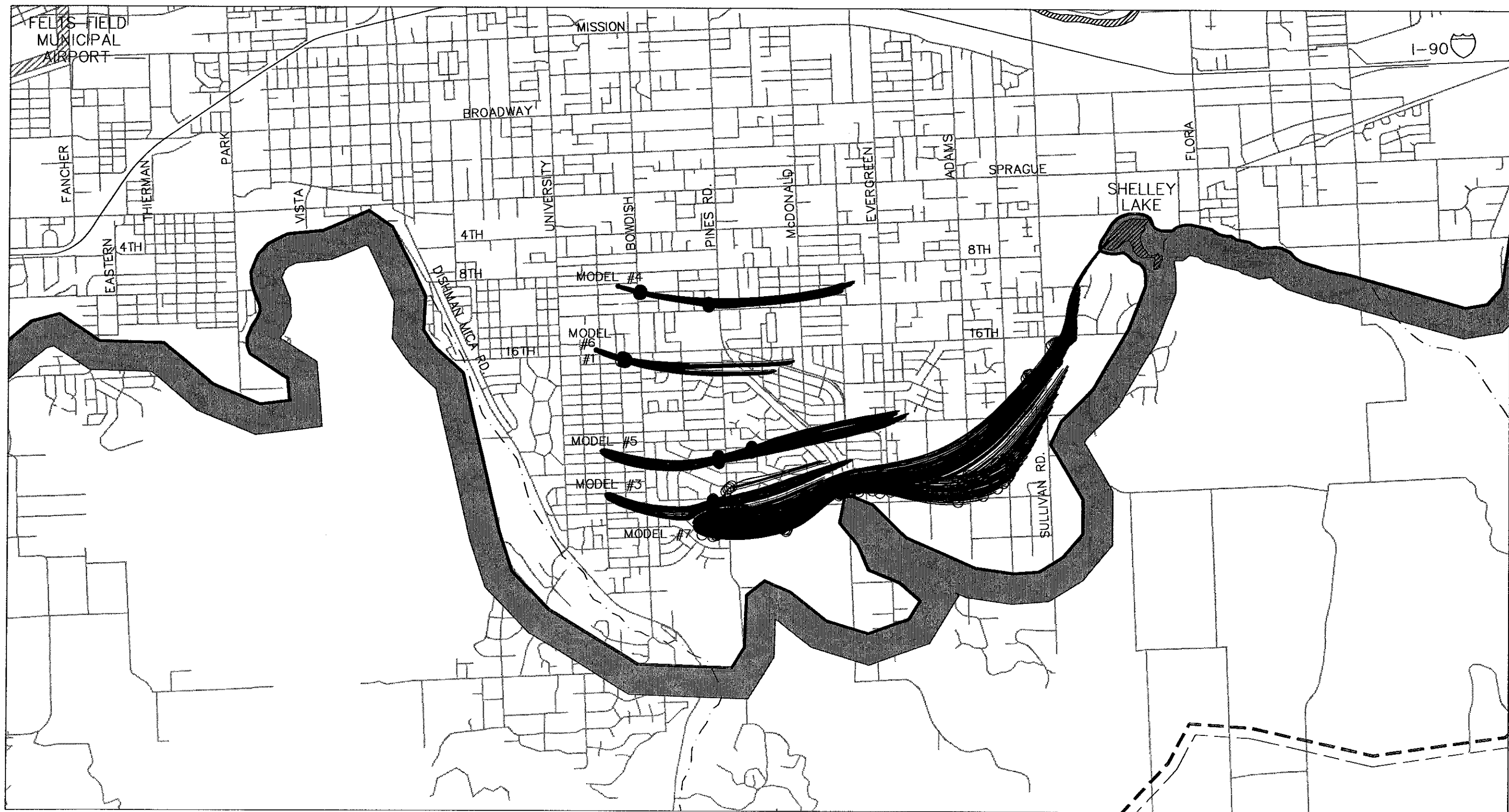
FIGURE 3-11 MODEL IRRIGATION DISTRICT NO. 18 PARTICLE TRACKING PLOT SPOKANE AQUIFER JOINT BOARD PROPOSED WELLHEAD PROTECTION AREAS AND DECEMBER 1997
