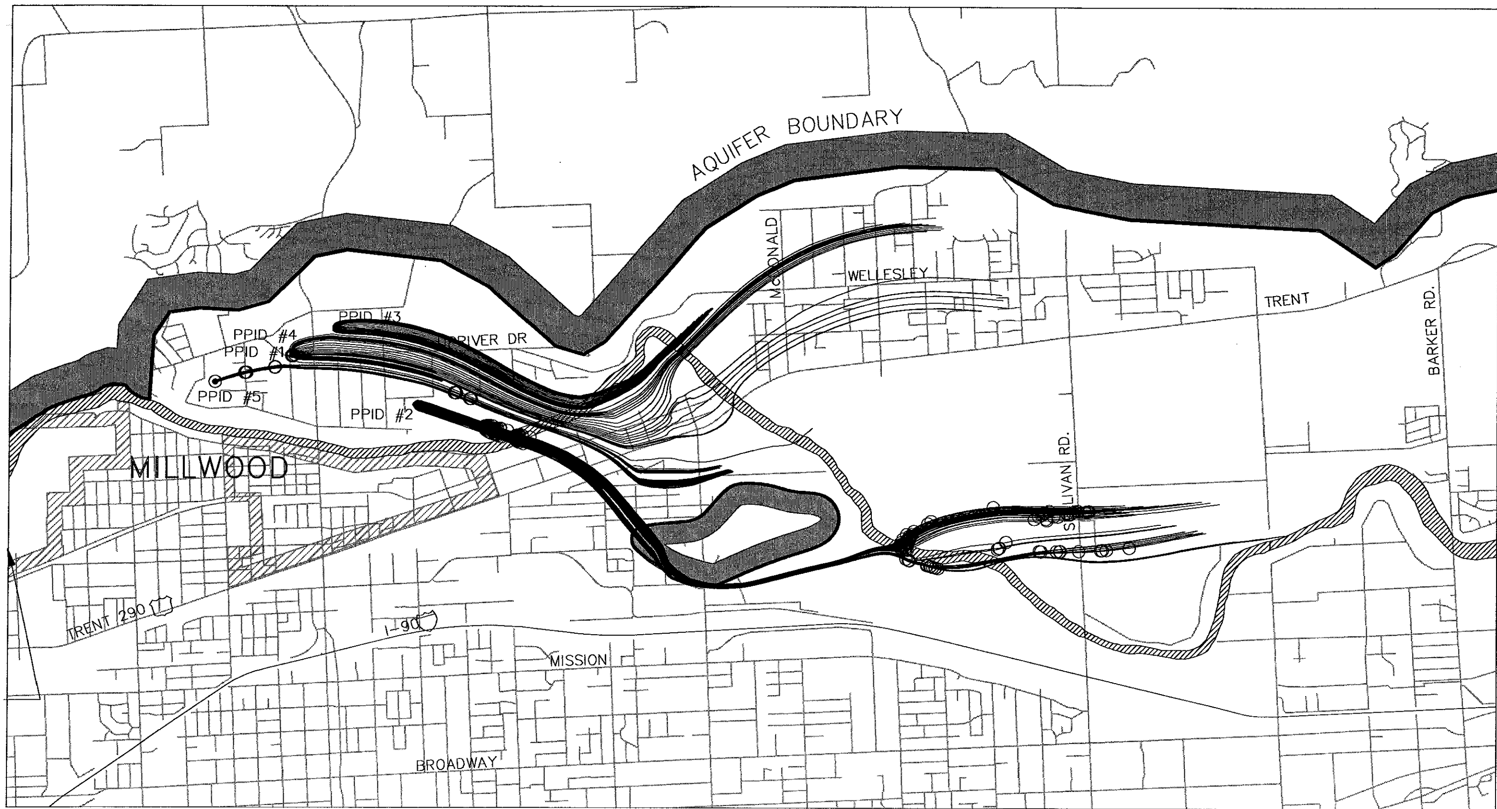
FIGURE 3-15 PASADENA PARK IRRIGATION DISTRICT NO. 17 PARTICLE TRACKING PLOT SPOKANE AQUIFER JOINT BOARD PROPOSED WELLHEAD PROTECTION AREAS AND DECEMBER 1997
