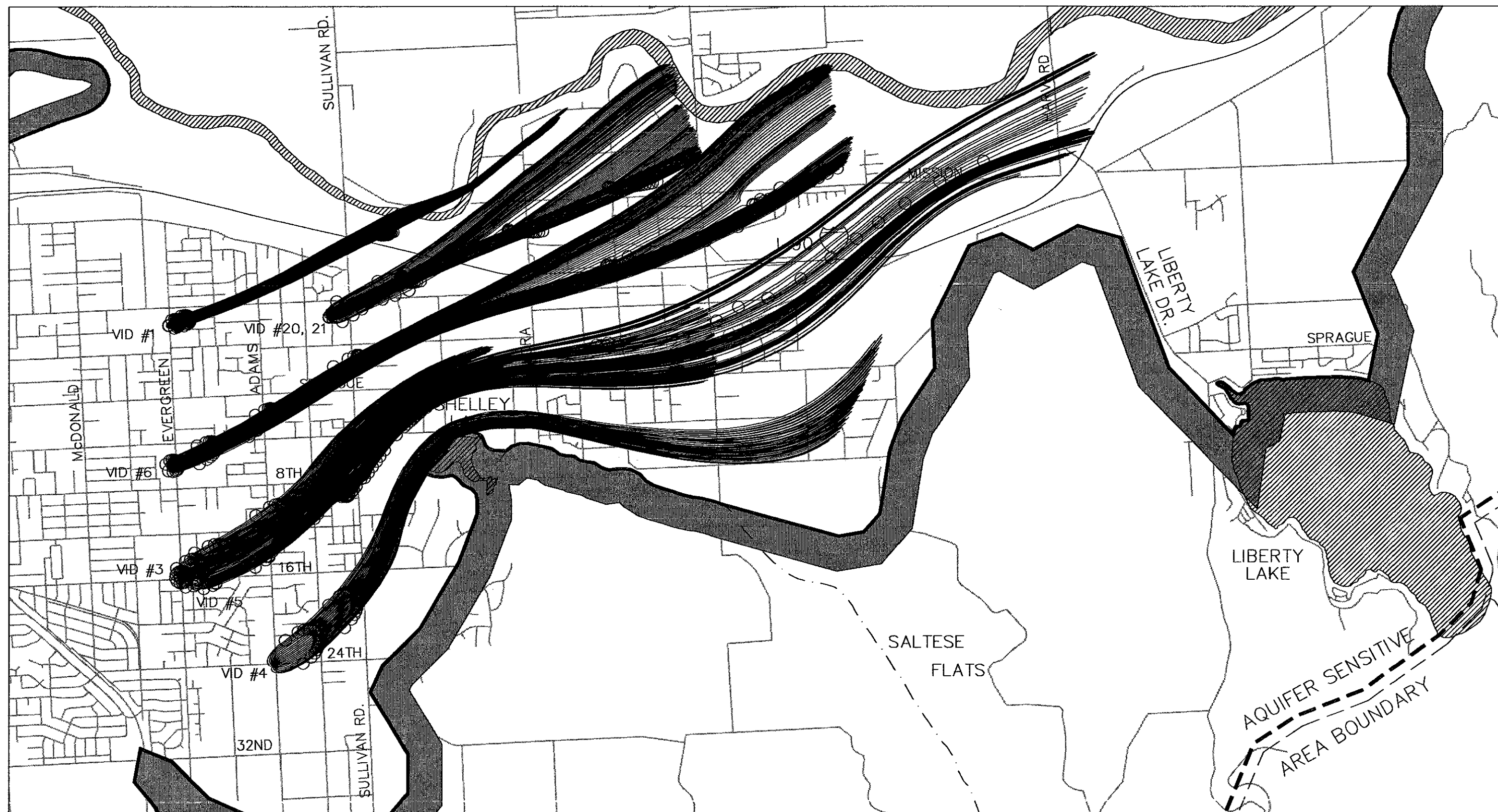
FIGURE 3-20 VERA WATER AND POWER PARTICLE TRACKING PLOT SPOKANE AQUIFER JOINT BOARD PROPOSED WELLHEAD PROTECTION AREAS AND DECEMBER 1997
