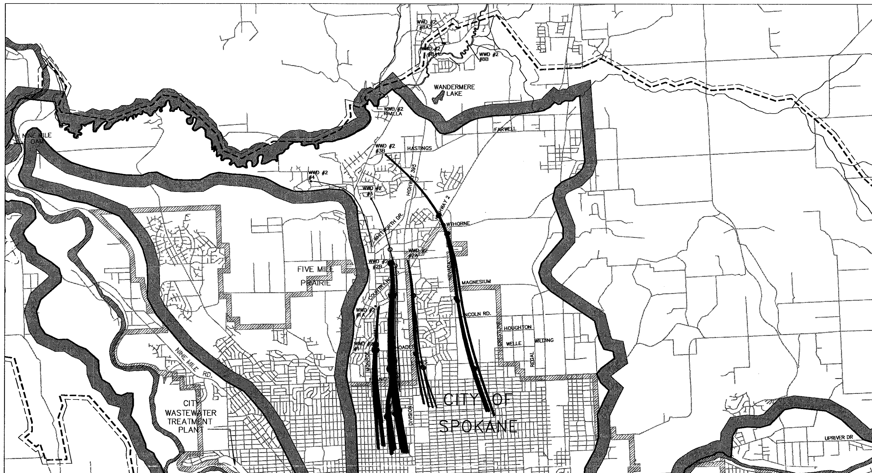
FIGURE 3-21 WHITWORTH WATER DISTRICT NO. 2 PARTICLE TRACKING PLOT SPOKANE AQUIFER JOINT BOARD PROPOSED WELLHEAD PROTECTION AREAS AND DECEMBER 1997
