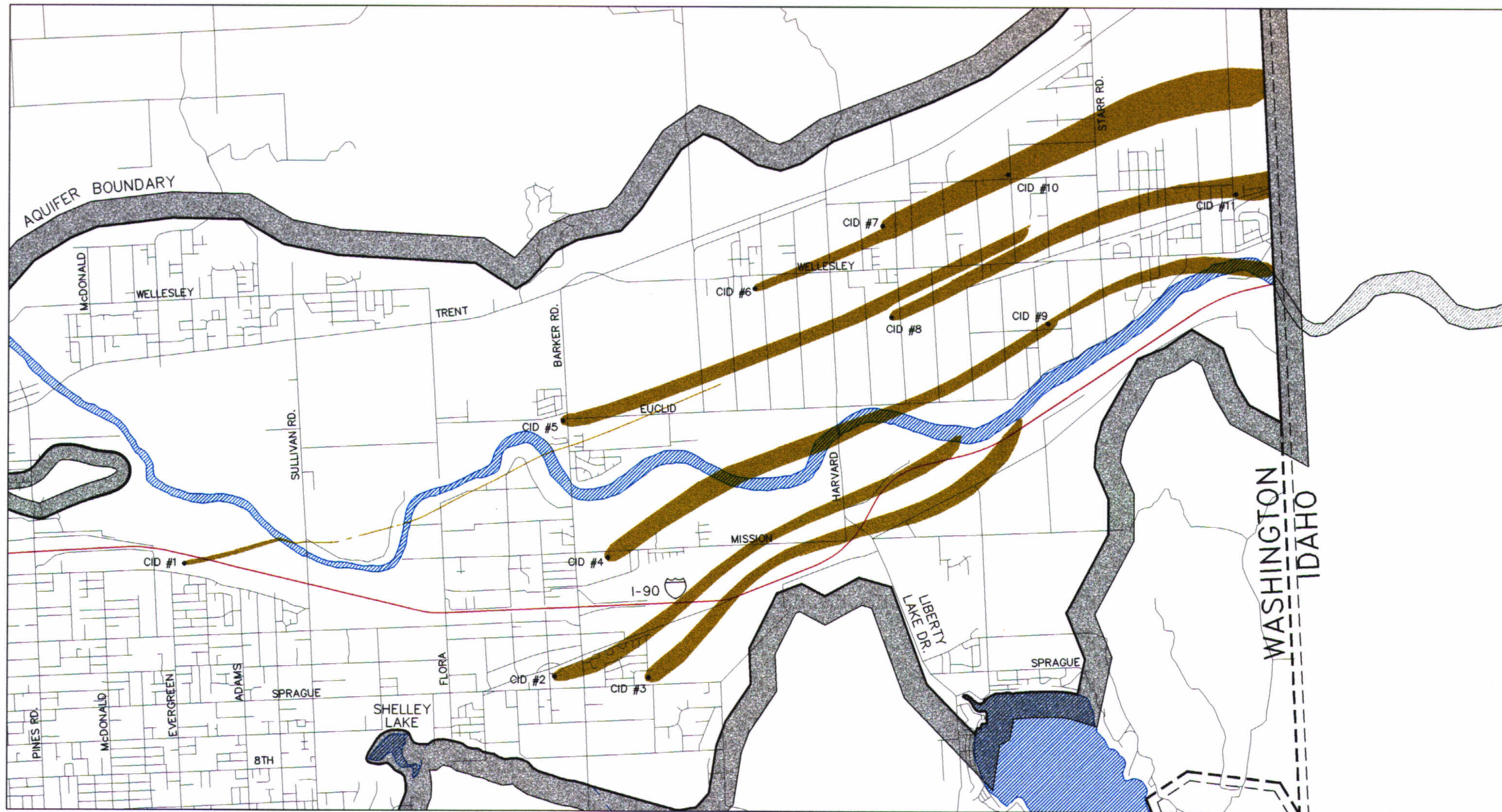
FIGURE 3-23 CONSOLIDATED IRRIGATION DISTRICT NO. 19 SPOKANE AQUIFER JOINT BOARD PROPOSED WELLHEAD PROTECTION AREAS DECEMBER 1997
