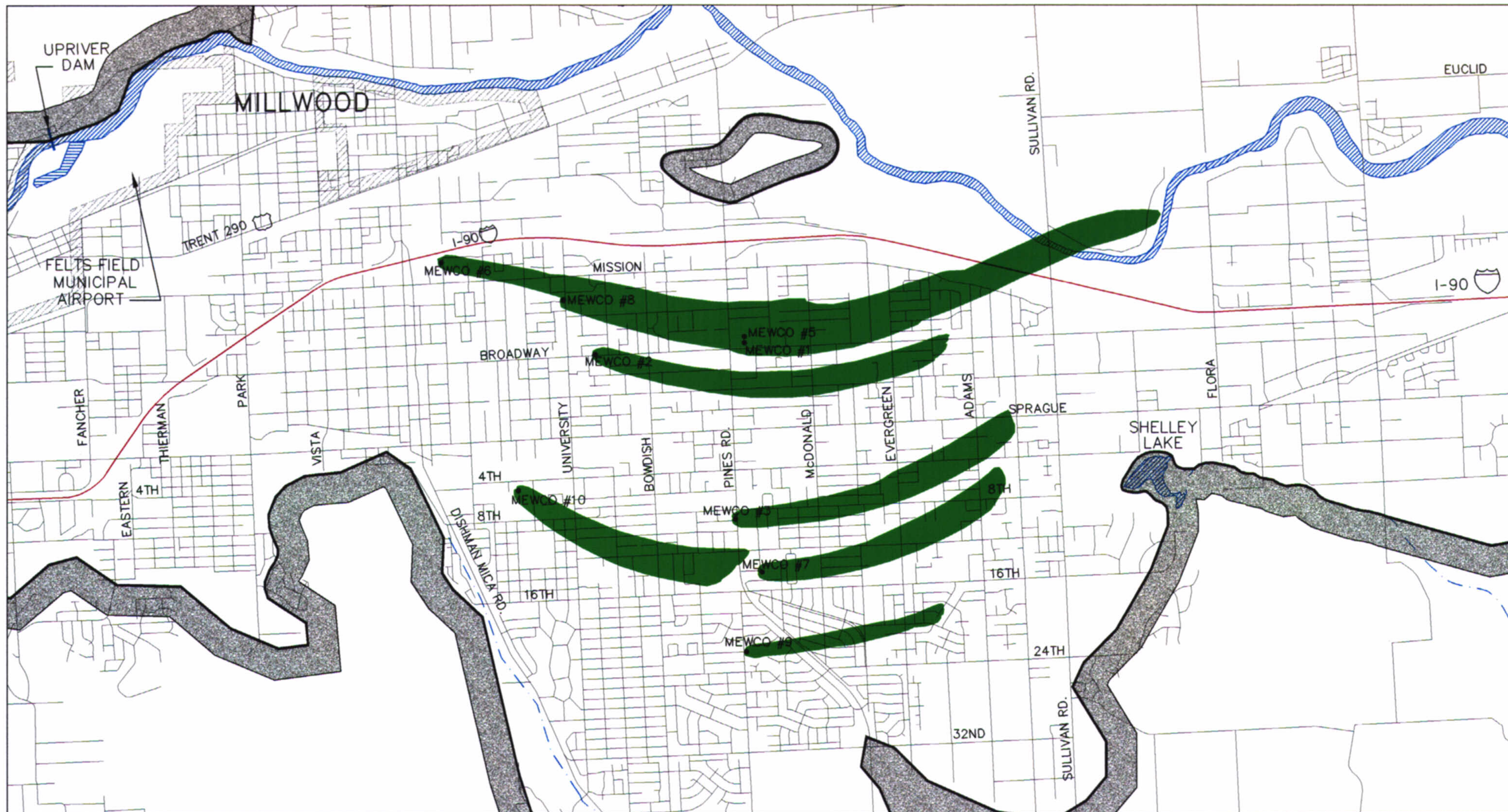
FIGURE 3-33 MODERN ELECTRIC WATER COMPANY SPOKANE AQUIFER JOINT BOARD PROPOSED WELLHEAD PROTECTION AREAS DECEMBER 1998
