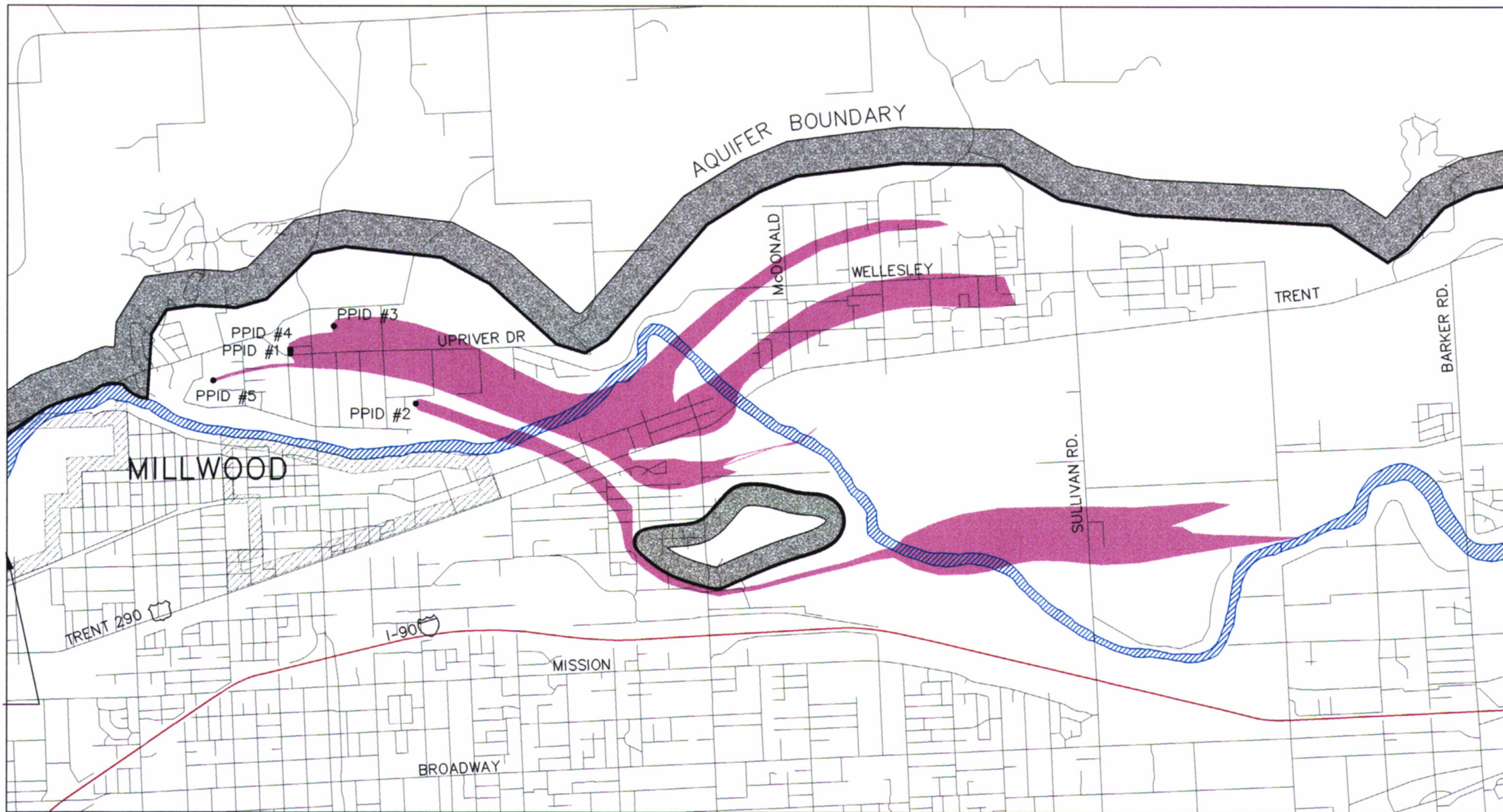
FIGURE 3-36 PASADENA PARK IRRIGATION DISTRICT NO. 17 SPOKANE AQUIFER JOINT BOARD PROPOSED WELLHEAD PROTECTION AREAS DECEMBER 1997
