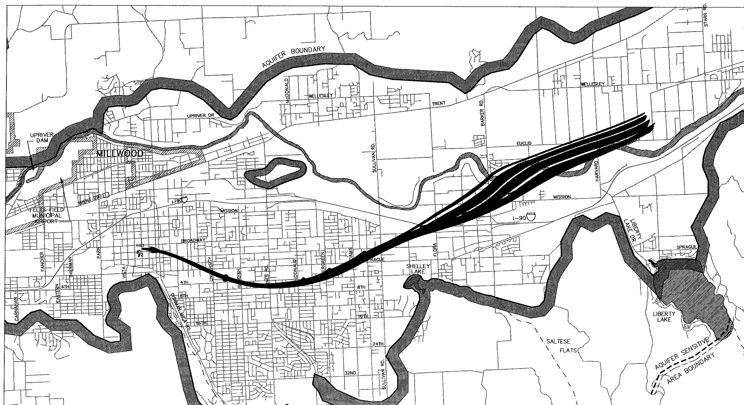
FIGURE 3-4 HUTCHINSON IRRIGATION DISTRICT NO. 16 PARTICLE TRACKING PLOT SPOKANE AQUIFER JOINT BOARD PROPOSED WELLHEAD PROTECTION AREAS AND DECEMBER 1997
