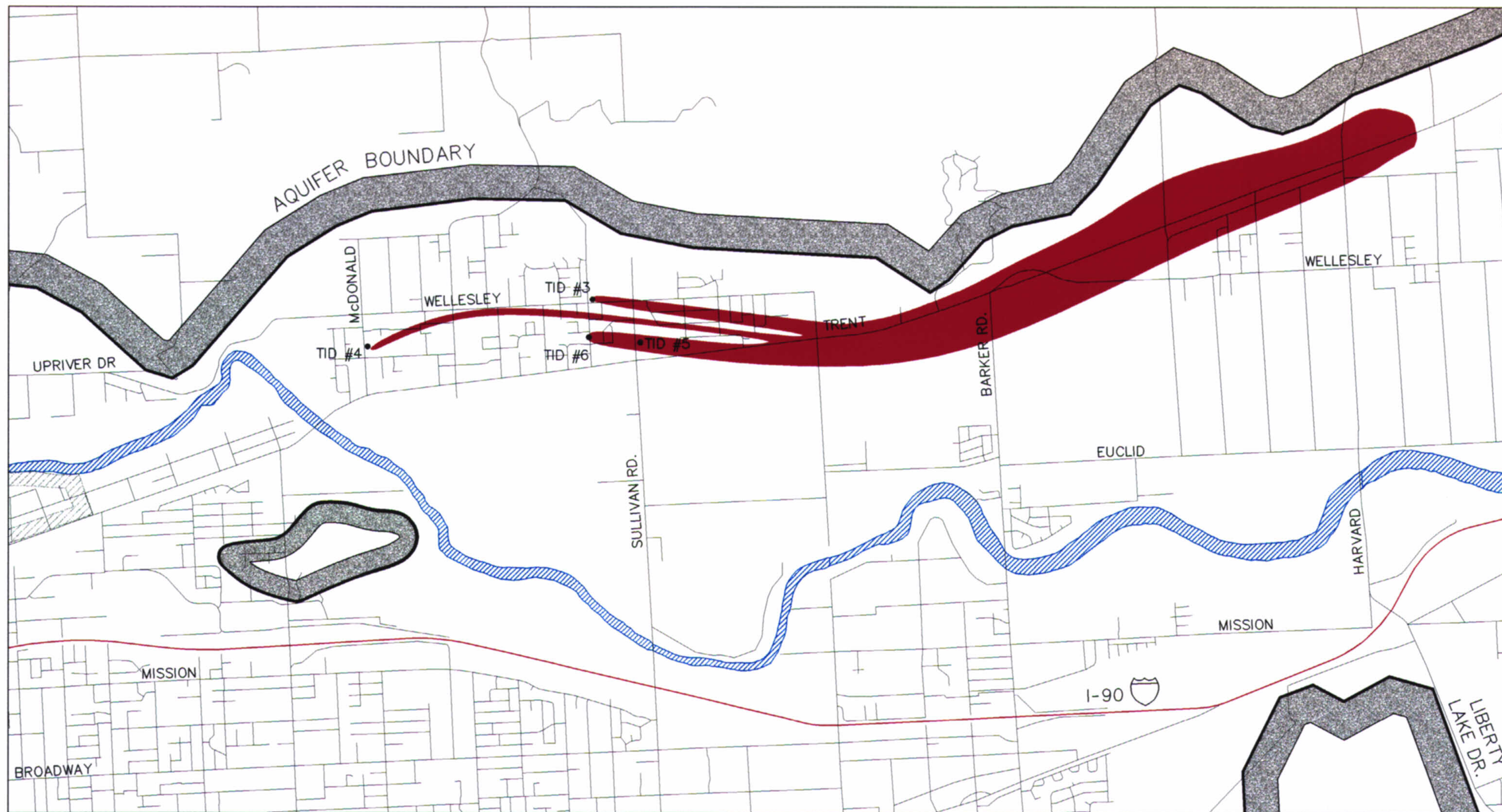
FIGURE 3-40 TRENTWOOD IRRIGATION DISTRICT NO. 3 SPOKANE AQUIFER JOINT BOARD PROPOSED WELLHEAD PROTECTION AREAS DECEMBER 1997
