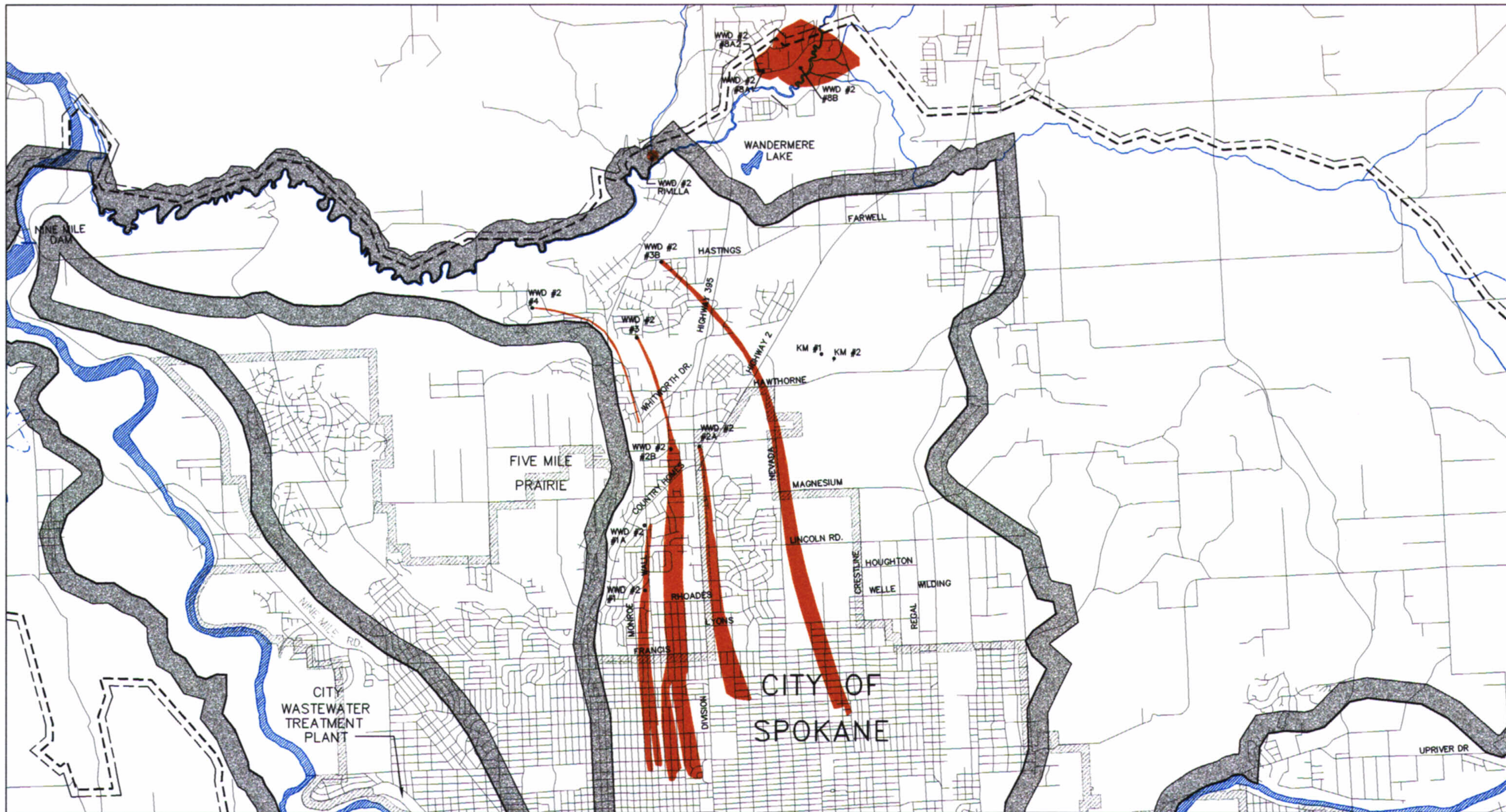
FIGURE 3-42 WHITWORTH WATER DISTRICT NO. 2 SPOKANE AQUIFER JOINT BOARD PROPOSED WELLHEAD PROTECTION AREAS DECEMBER 1997
