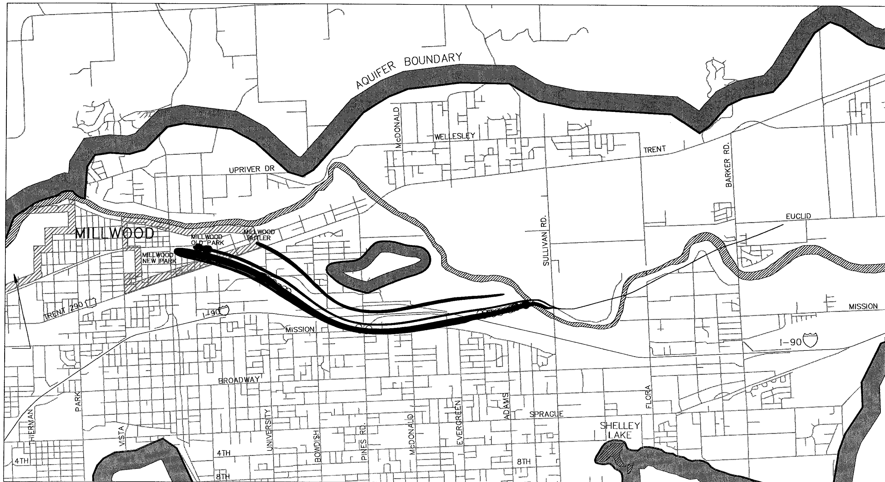
FIGURE 3-9 TOWN OF MILLWOOD PARTICLE TRACKING PLOT SPOKANE AQUIFER JOINT BOARD PROPOSED WELLHEAD PROTECTION AREAS AND DECEMBER 1997
