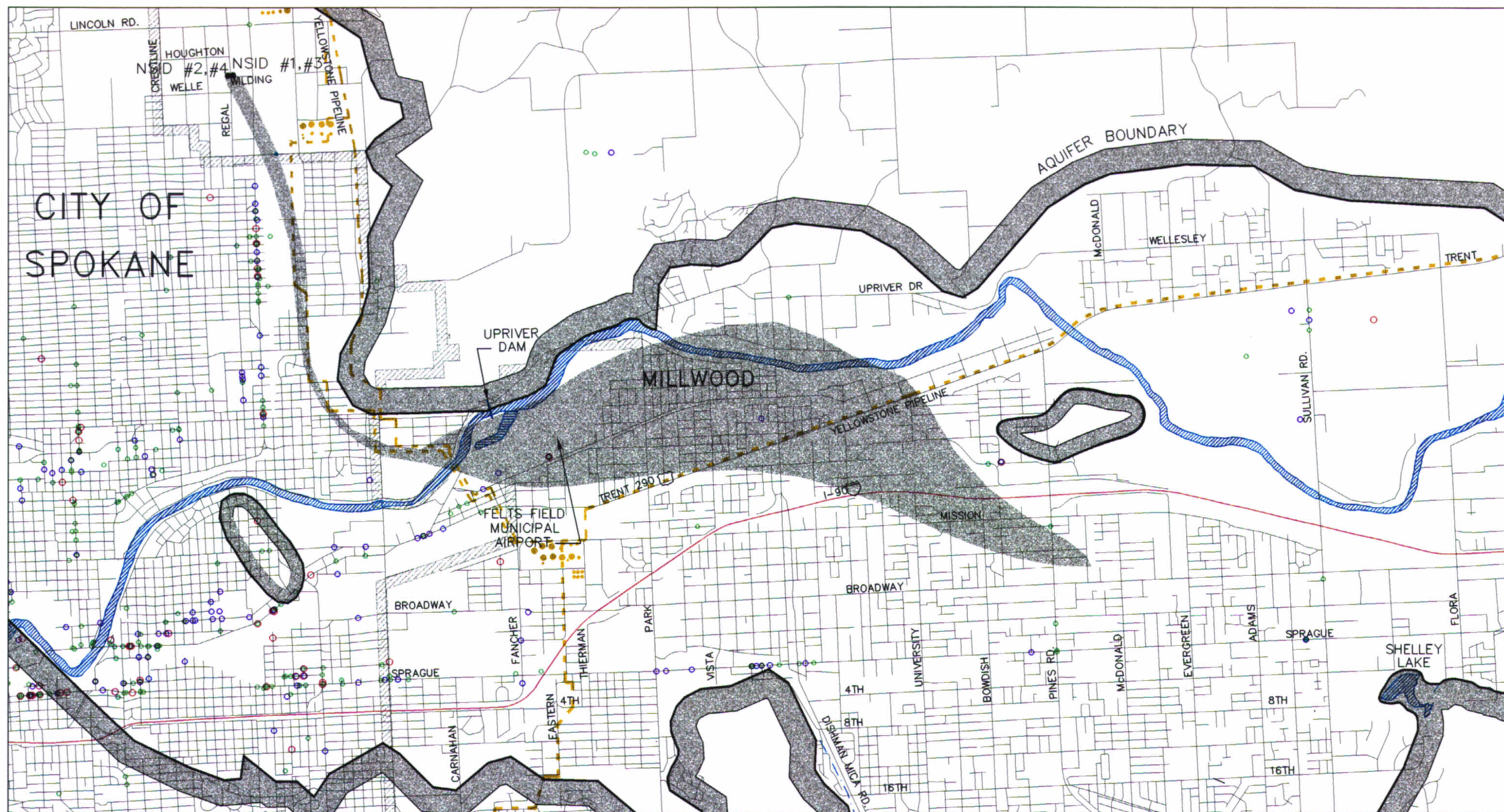
FIGURE 6-13B NORTH SPOKANE IRRIGATION DISTRICT NO. 8 SPOKANE AQUIFER JOINT BOARD PROPOSED WELLHEAD PROTECTION AREAS AND POTENTIAL HISTORICAL CONTAMINANT SOURCES DECEMBER 1997
