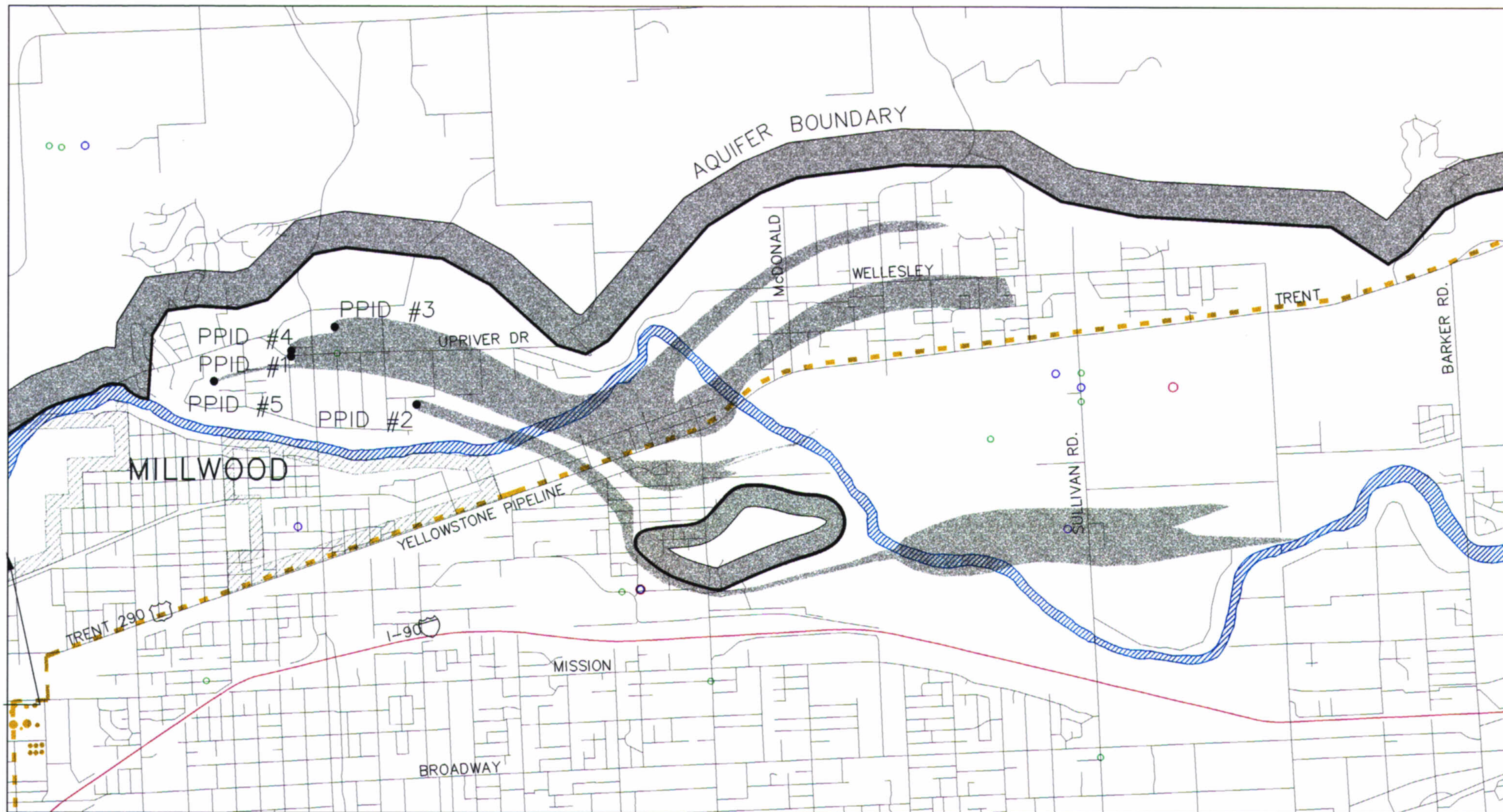
FIGURE 6-15B PASADENA PARK IRRIGATION DISTRICT NO. 17 SPOKANE AQUIFER JOINT BOARD PROPOSED WELLHEAD PROTECTION AREAS AND POTENTIAL HISTORICAL CONTAMINANT SOURCES DECEMBER 1997
