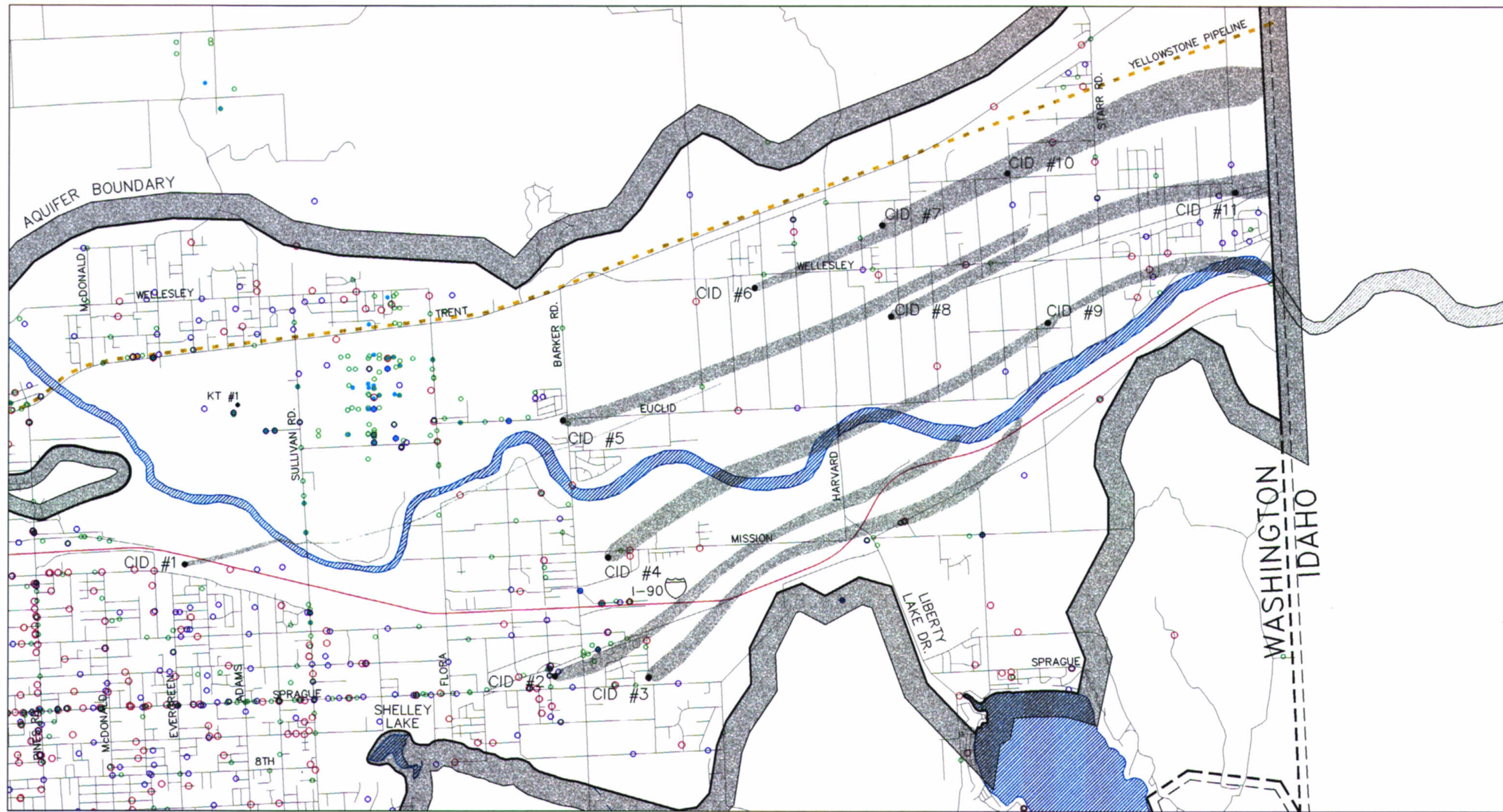
FIGURE 6-2A CONSOLIDATED IRRIGATION DISTRICT NO. 19 SPOKANE AQUIFER JOINT BOARD PROPOSED WELLHEAD PROTECTION AREAS AND POTENTIAL CURRENT CONTAMINANT SOURCES DECEMBER 1997
