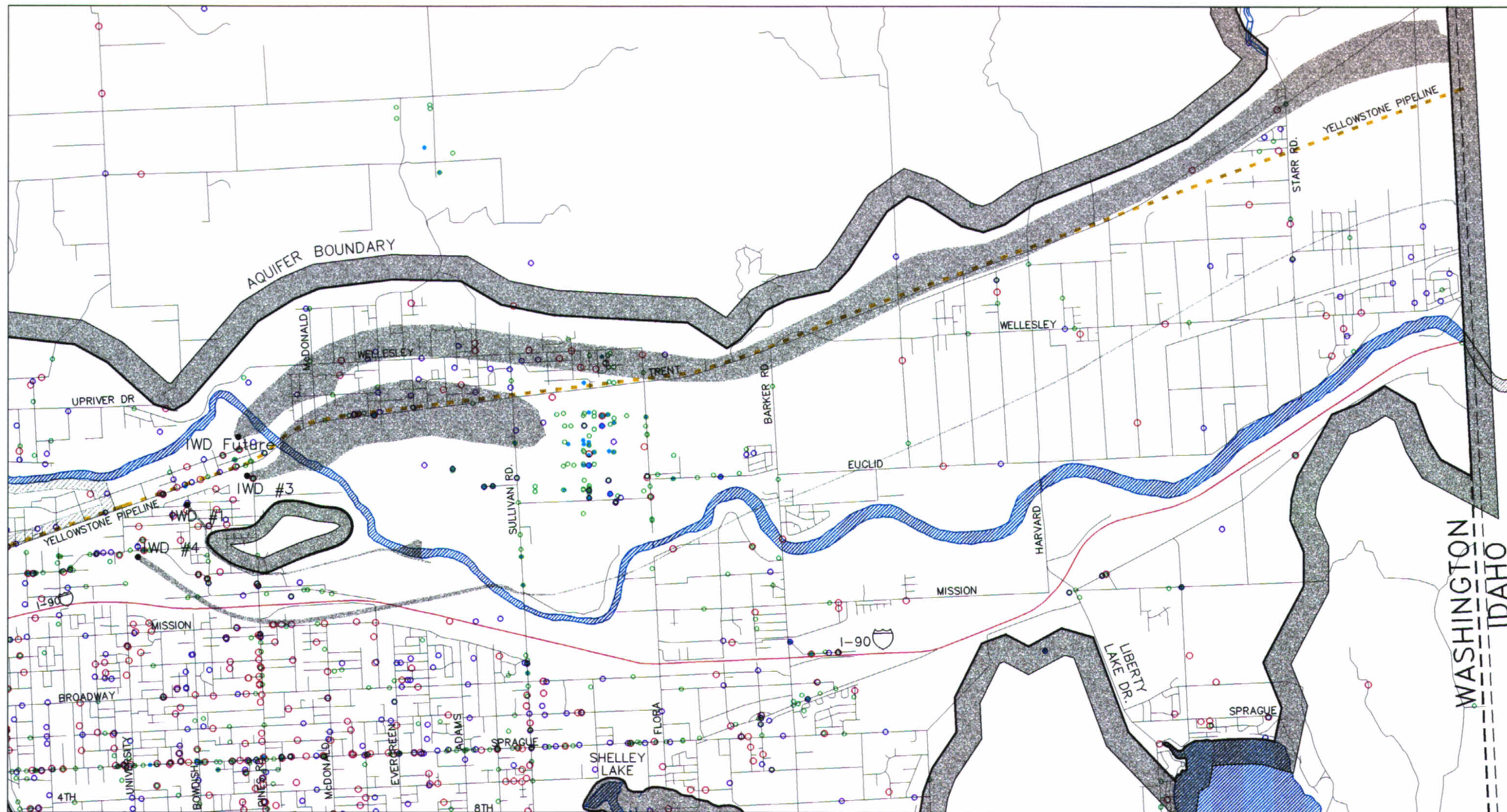
FIGURE 6-5A IRVIN WATER DISTRICT NO. 6 SPOKANE AQUIFER JOINT BOARD PROPOSED WELLHEAD PROTECTION AREAS AND POTENTIAL CURRENT CONTAMINANT SOURCES DECEMBER 1997
