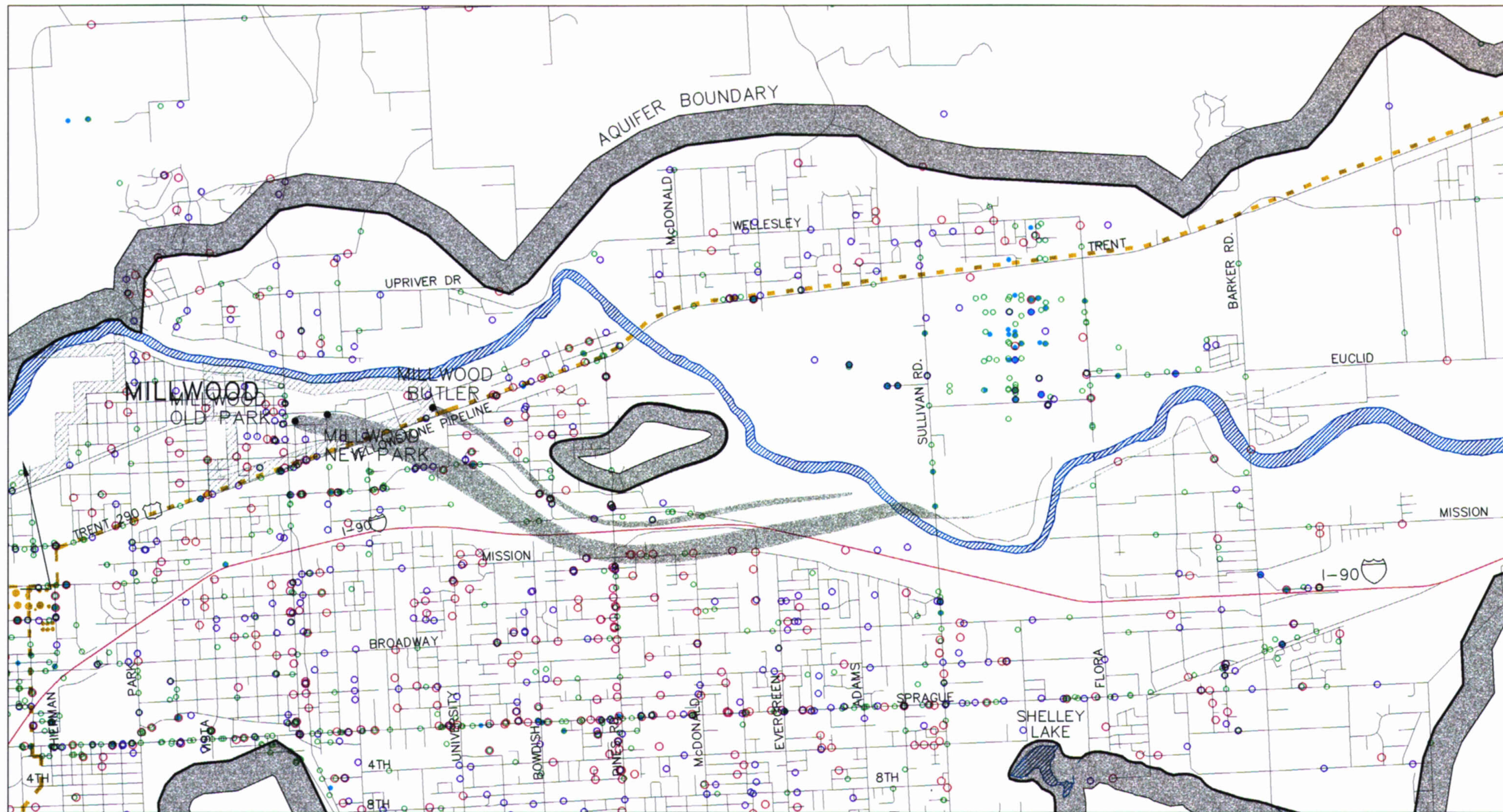
FIGURE 6-9A TOWN OF MILLWOOD SPOKANE AQUIFER JOINT BOARD PROPOSED WELLHEAD PROTECTION AREAS AND POTENTIAL CURRENT CONTAMINANT SOURCES DECEMBER 1997
