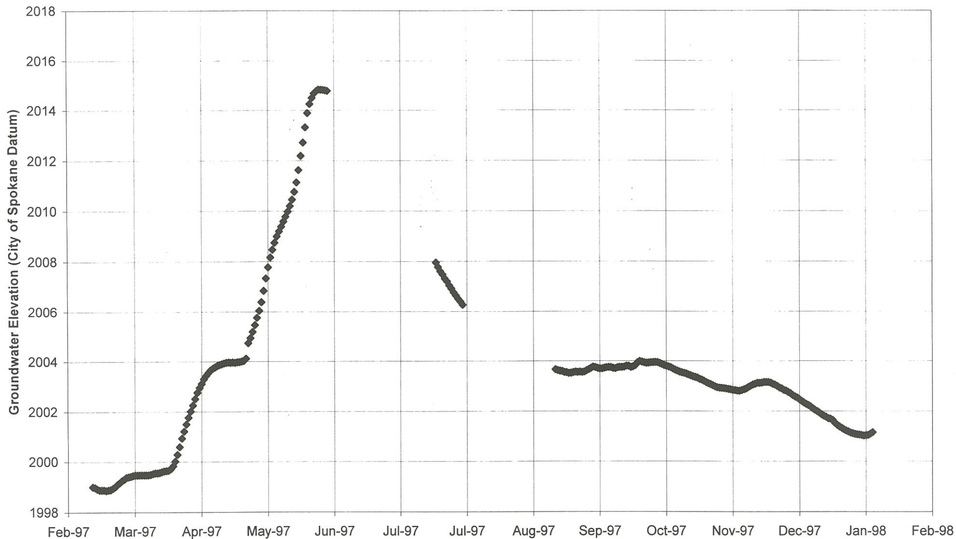
FIGURE 2-3 IDAHO ROAD MONITORING WELL GROUNDWATER ELEVATIONS FEBRUARY 1997 - FEBRUARY 1998 SPOKANE AQUIFER JOINT BOARD FEBRUARY 1998
